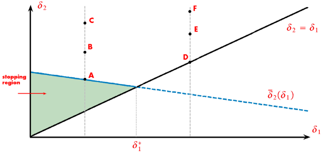
Figure 2: Optimal Policy
