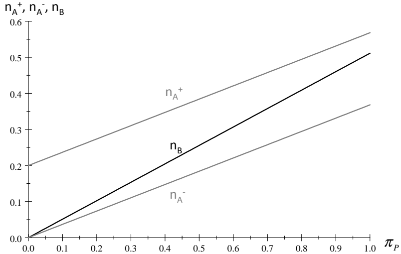
Figure 2: Investment as function of beliefs
