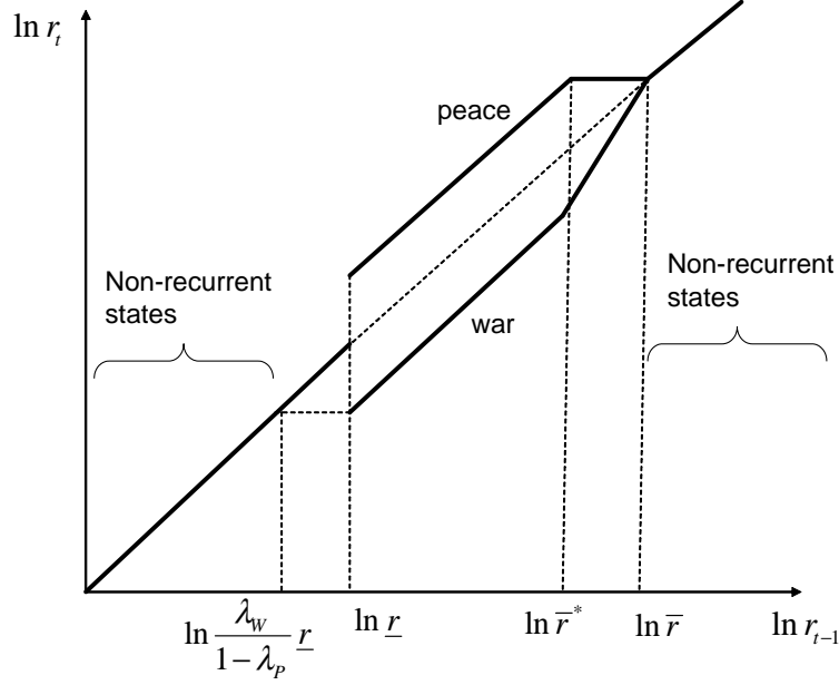
Figure 6: Dynamics of beliefs with two traps
