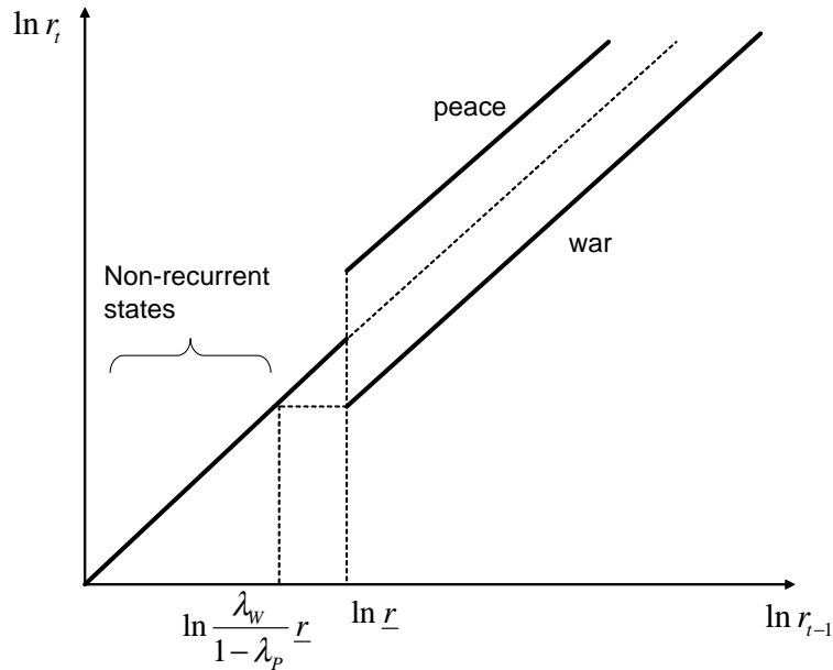
Figure 4: Dynamics of beliefs
