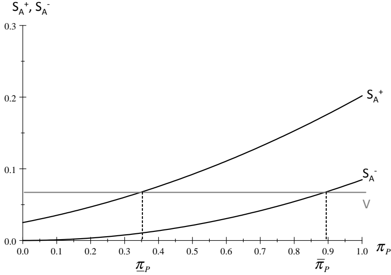
Figure 5: Surplus from trade and gains from war as function of beliefs in the presence of two traps
