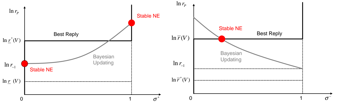
Figure 8: Multiple PBE and Mixed-Strategy PBE
