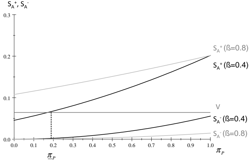
Figure 7: Surplus from trade with exogenous \beta
