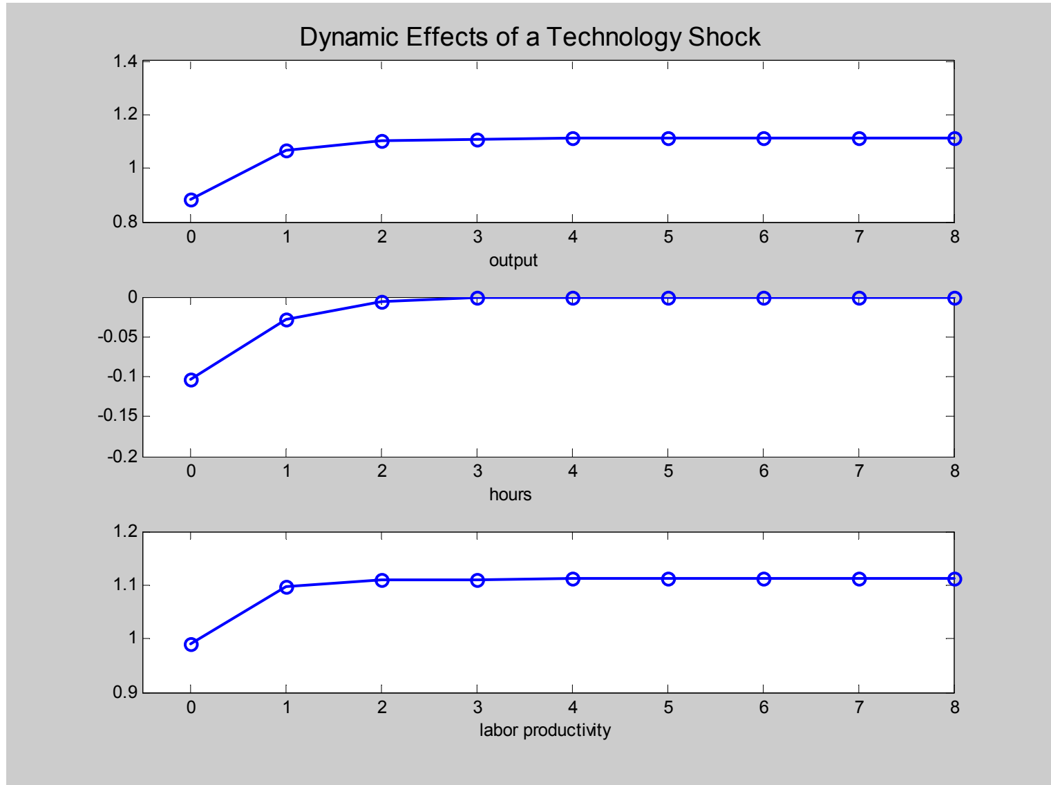
Figure 16 Pre-84 Calibration: Technology Shock
