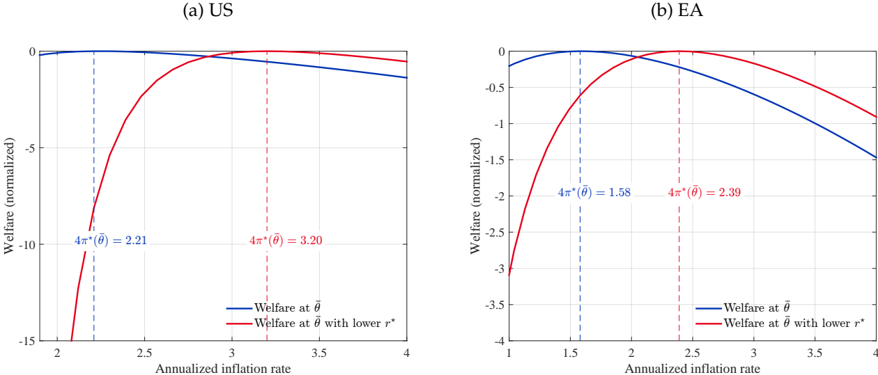
Figure C.1: \mathcal{W}(\pi, \mathbb{E}(\theta))
