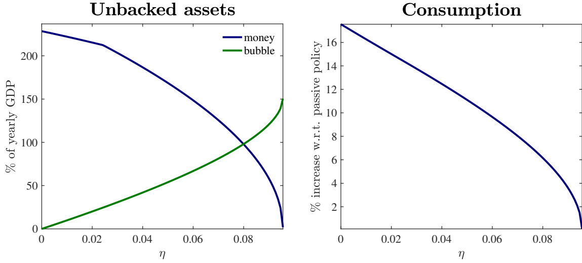
FIGURE 10: Illustrates how the steady-state values of private bubbles, money and consumption vary with bubble-creation, under optimal monetary policy, in our calibrated economy.
