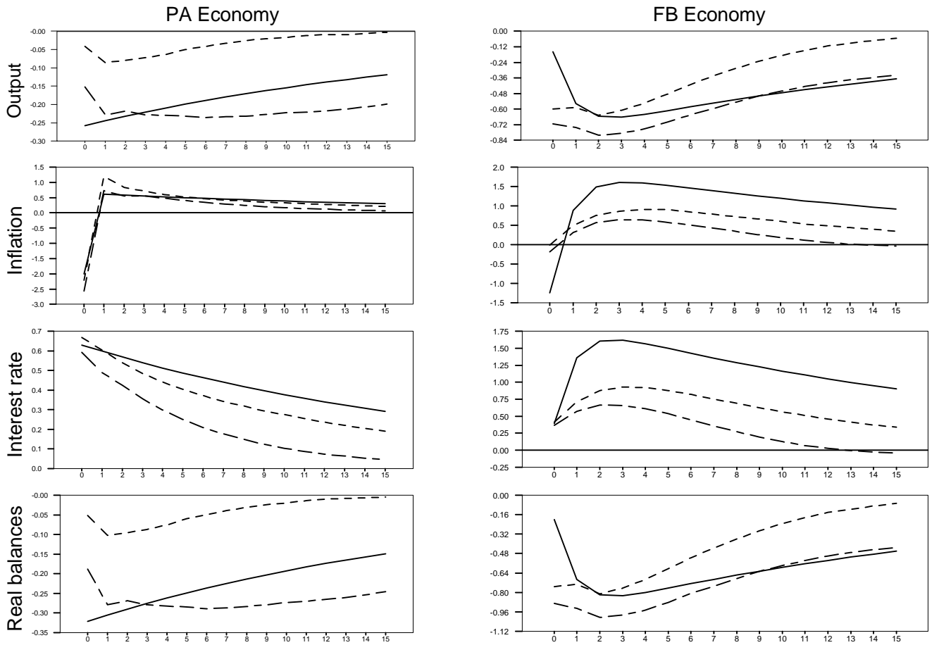
Estimated Impulse Response Bands, SIMS92 Identification
